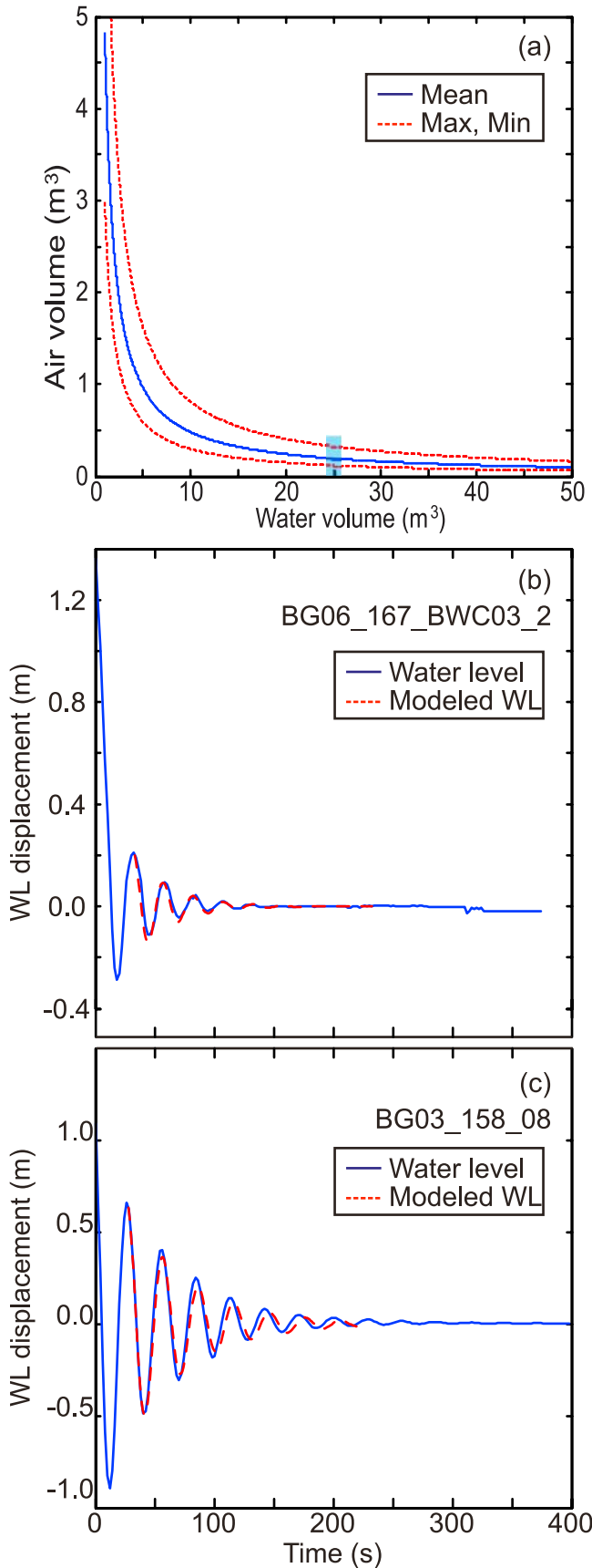
Figure 7. (a) Model results show that as water volume increases, the volume of air needed to produce oscillations with the range of observed frequencies declines exponentially. Application of the model to two slug test results from (b) 2006 and (c) 2003, respectively, show a good fit for calculated air volumes given a water volume of 25 \text{ m}^3 (shaded box in Figure 7a). Timescales are consistent for Figures 7b and 7c. Calculated air volumes for Figures 7b and 7c are 0.11 and 0.16 \text{ m}^3 , respectively.
